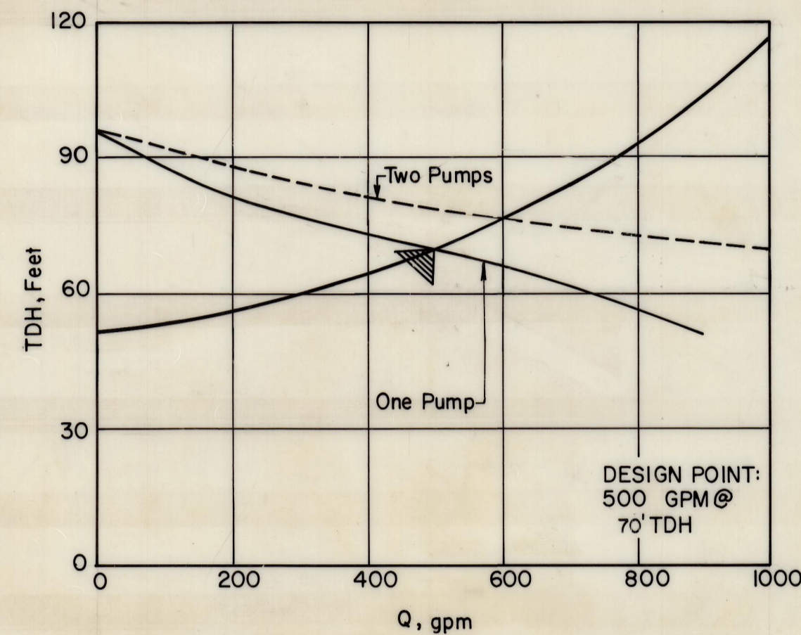
PUMPING STATION NO. 3-2
