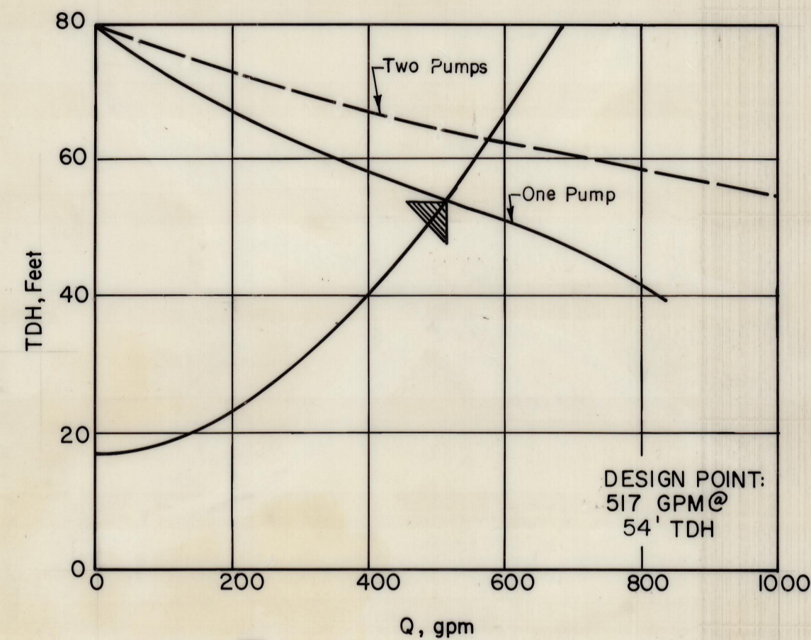
PUMPING STATION NO. 6-1
