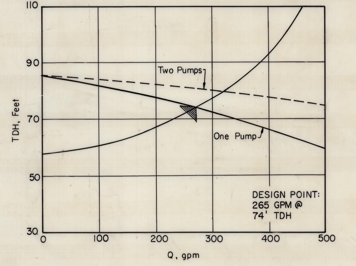
PUMPING STATION NO. 5-1
