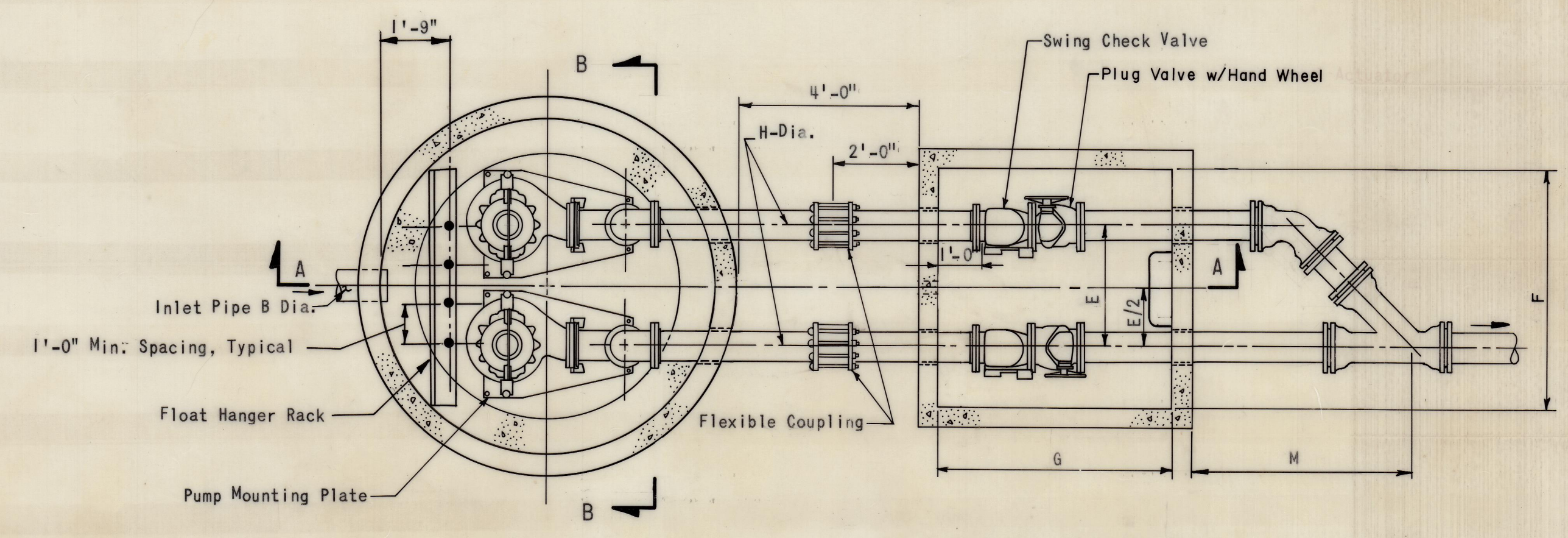
PLAN - TOP SLABS REMOVED
