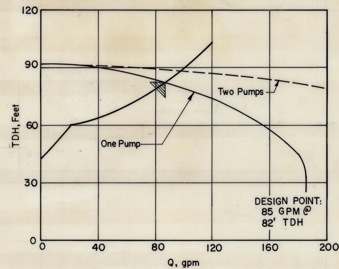
PUMPING STATION NO. 8-1
