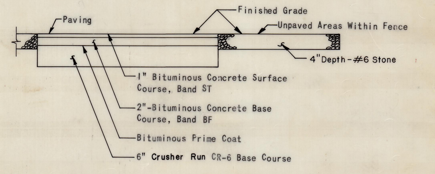
TYPICAL PAVING SECTION
