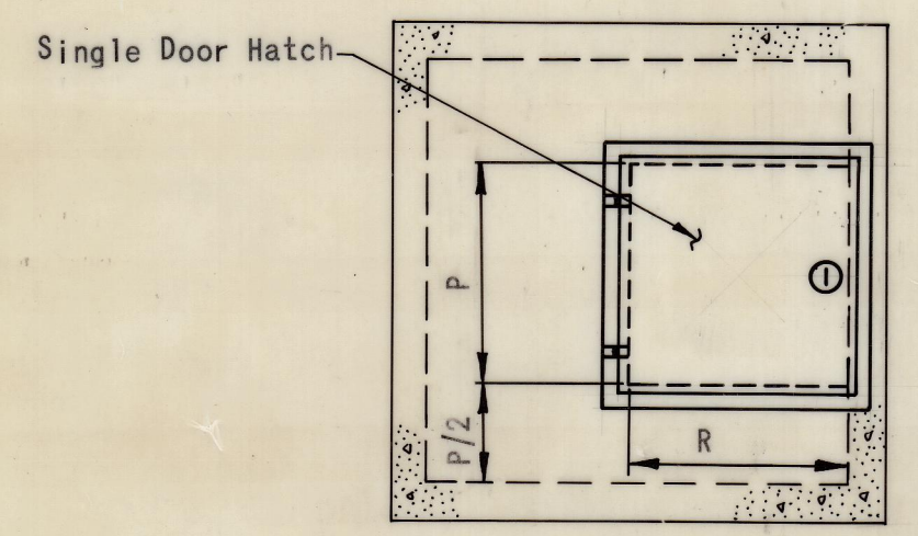
PLAN - TOP SLAB, VALVE VAULT
