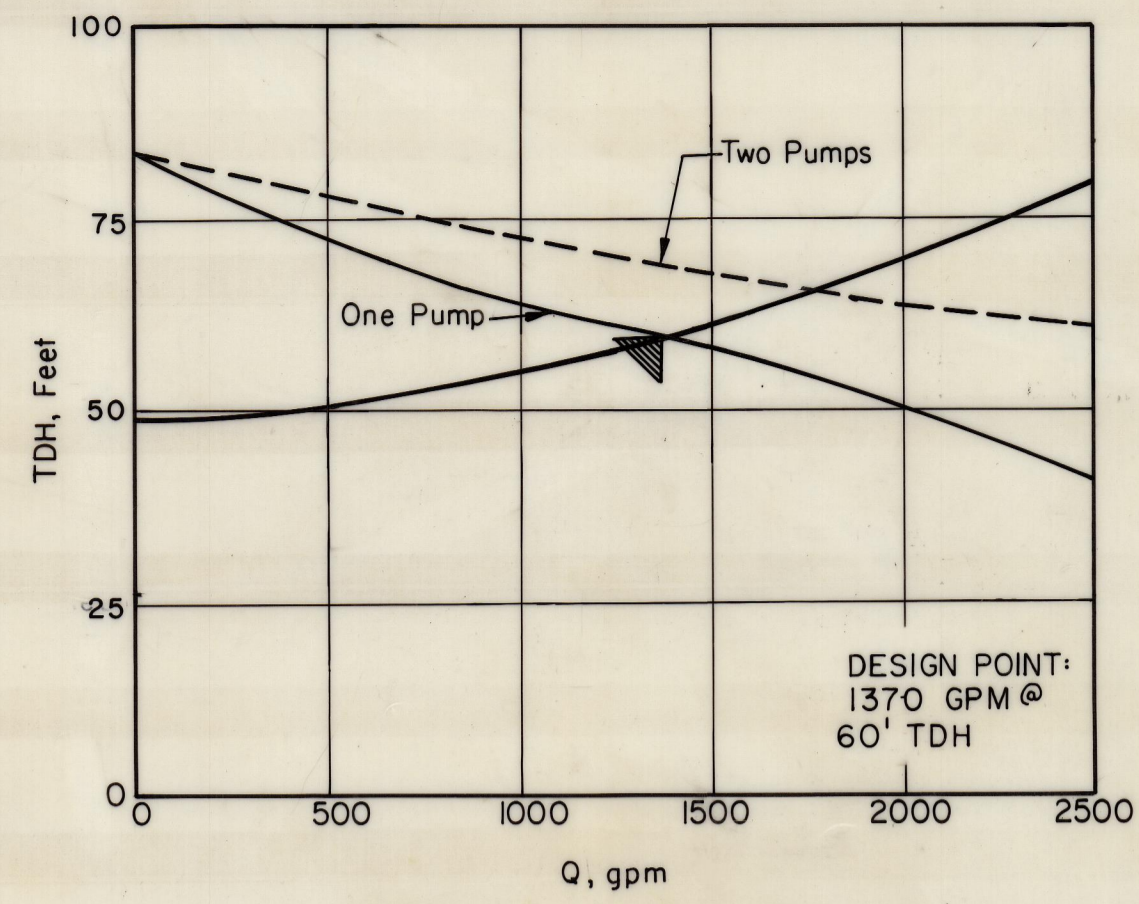
PUMPING STATION NO. 1-1
