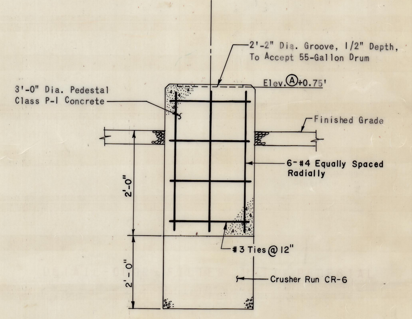
DETAIL - ODOR FILTER UNIT PEDESTAL
