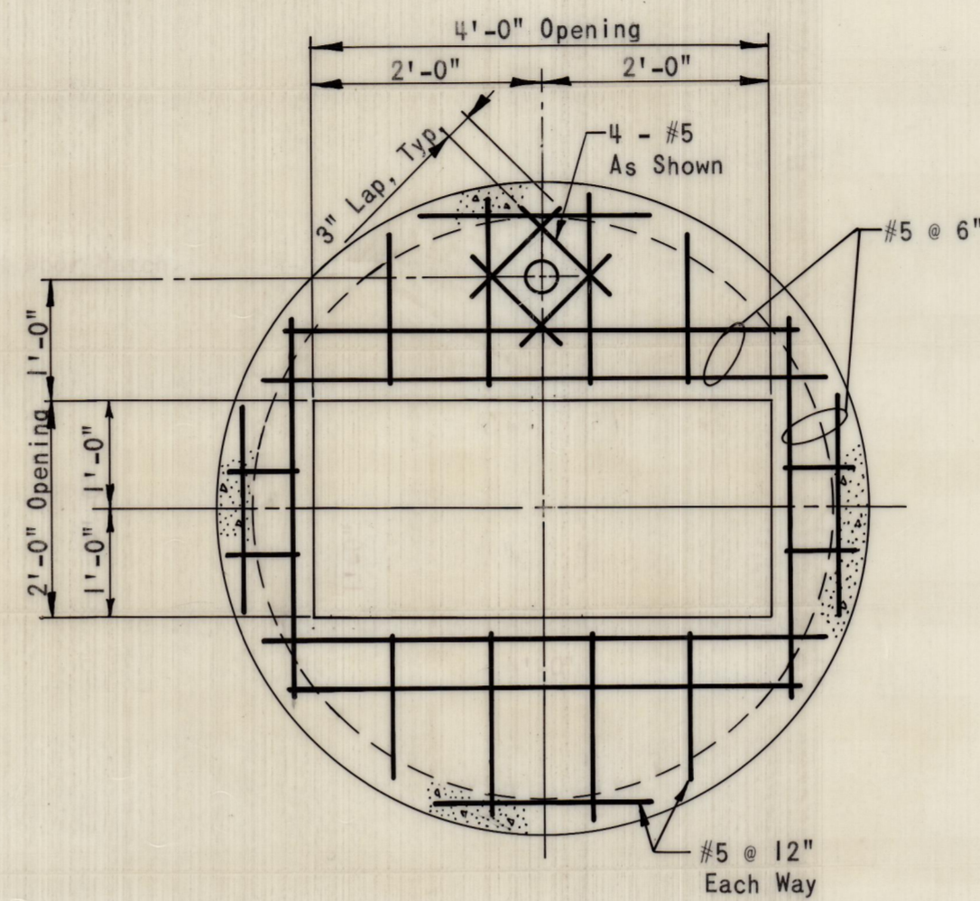
PLAN - TOP SLAB, PUMPING STATION
