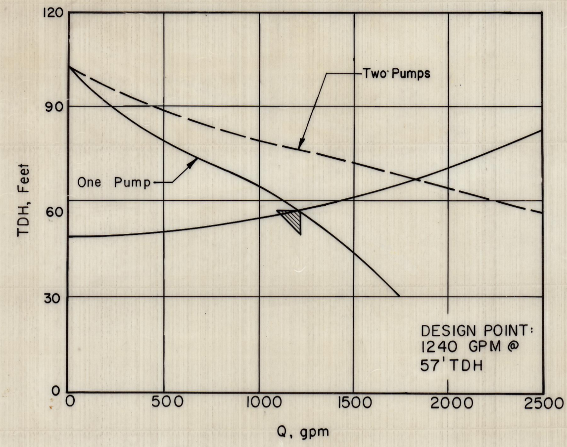
PUMPING STATION NO. 2-2
