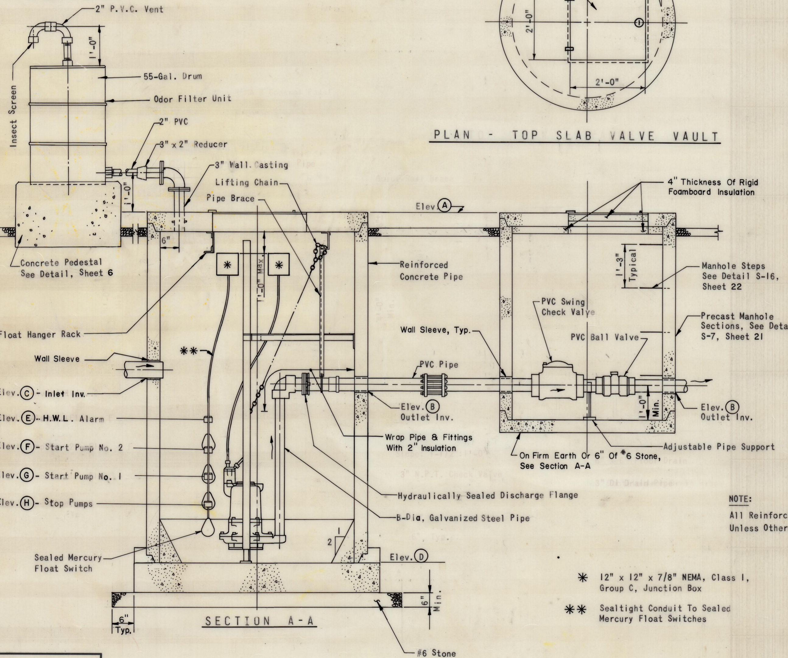
PUMPING STATION AND VALVE VAULT DETAILS
