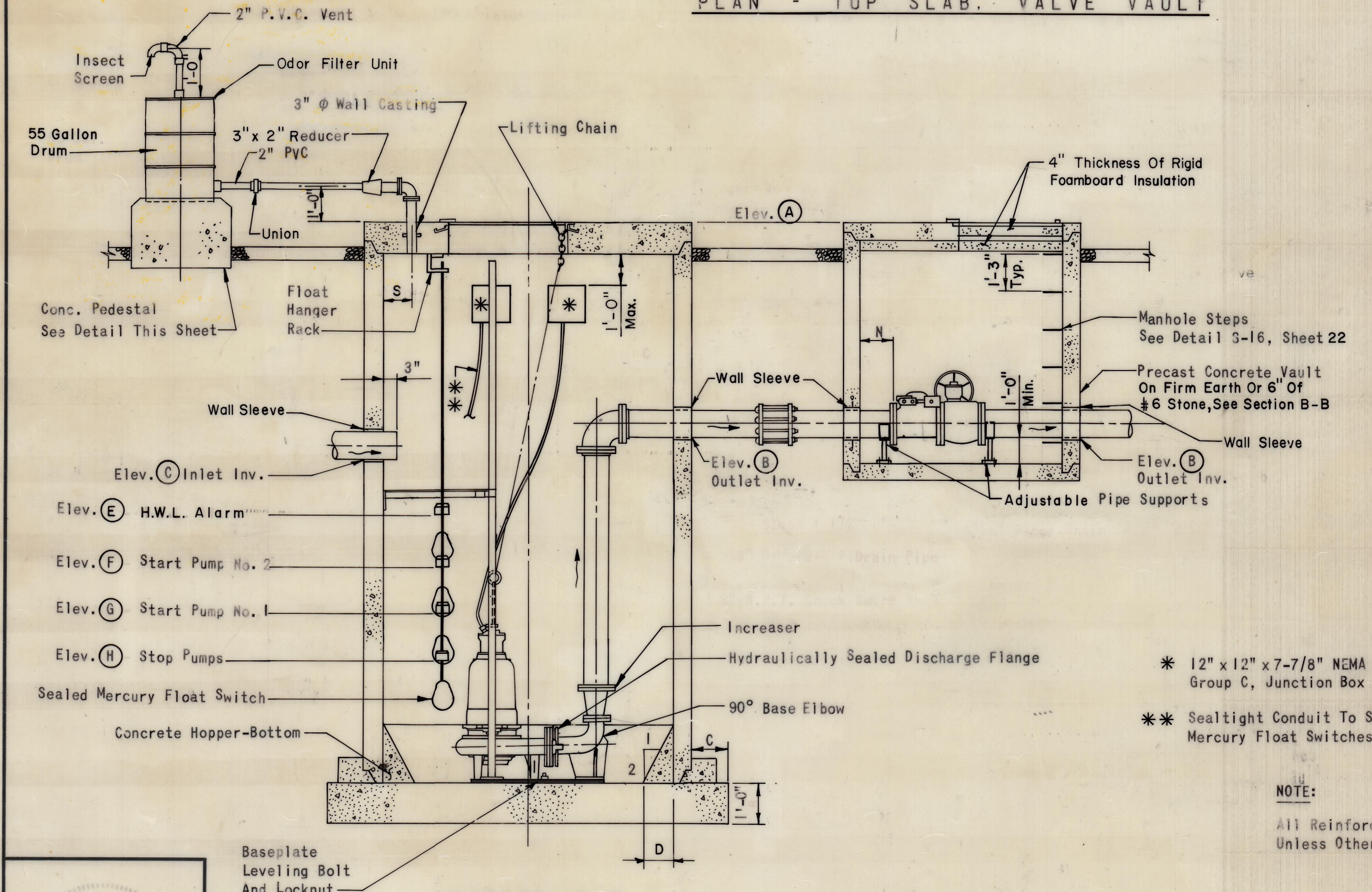
PUMPING STATION AND VALVE VAULT DETAILS
