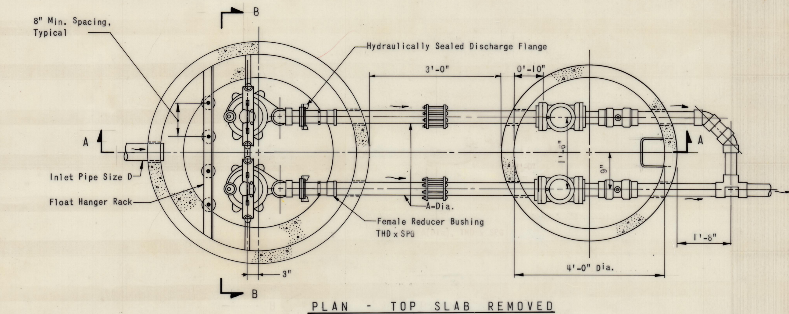
PLAN - TOP SLAB REMOVED
