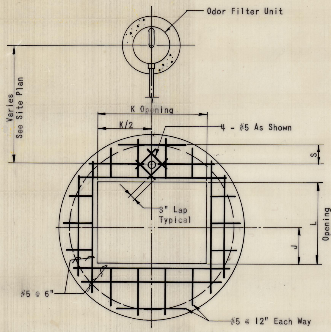
PLAN - TOP SLAB, PUMPING STATION
