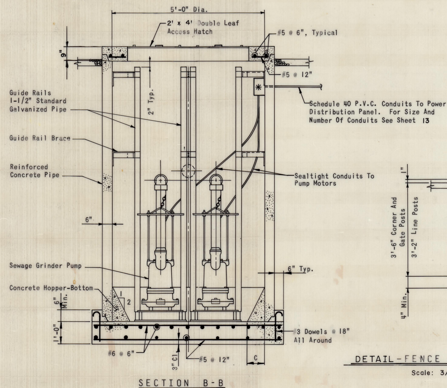
SECTION B-B
